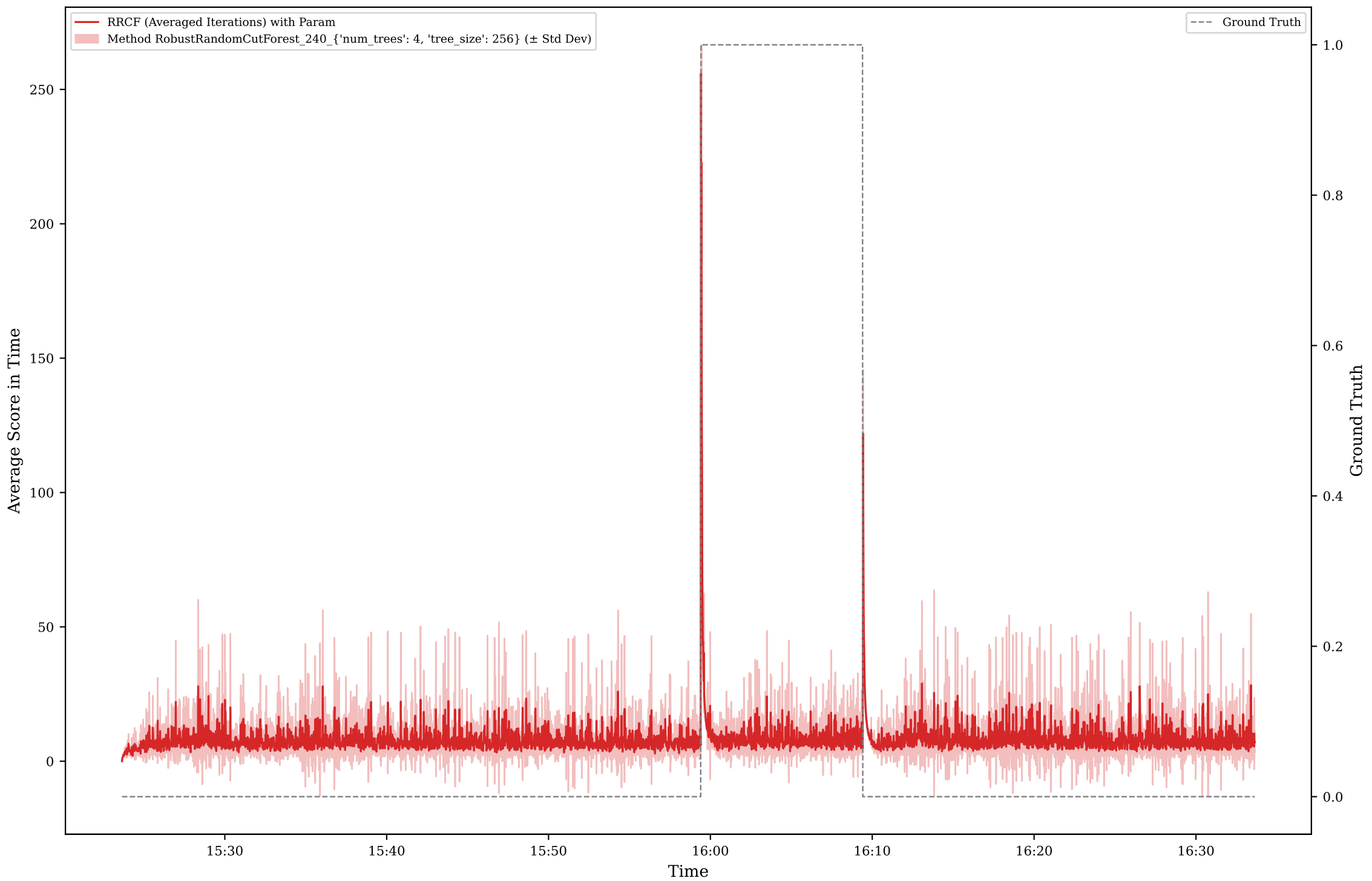
Method RRCF Score for Scenario A3
